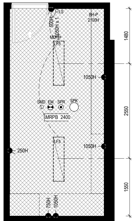
6 RCP-TREATMENT Scale 1 : 50
