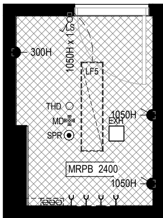
2 RCP-CLEANER - TYPE 1 Scale 1 : 50
