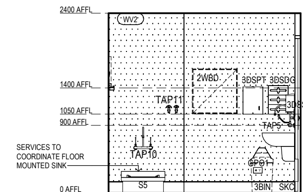
RACF BOH - CLEANER - TYPE 1 ELEVATION 4 Scale 1 : 50
