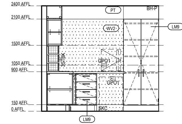
RACF BOH - TREATMENT ELEVATION 3 Scale 1 : 50
