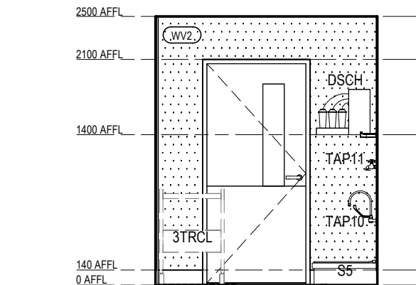
RACF BOH - CLEANER - TYPE 2 ELEVATION 4 Scale 1 : 50
