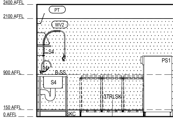
RACF BOH - SLUICE ELEVATION 2 Scale 1 : 50
